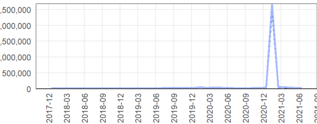
21: RAWDATA staging
